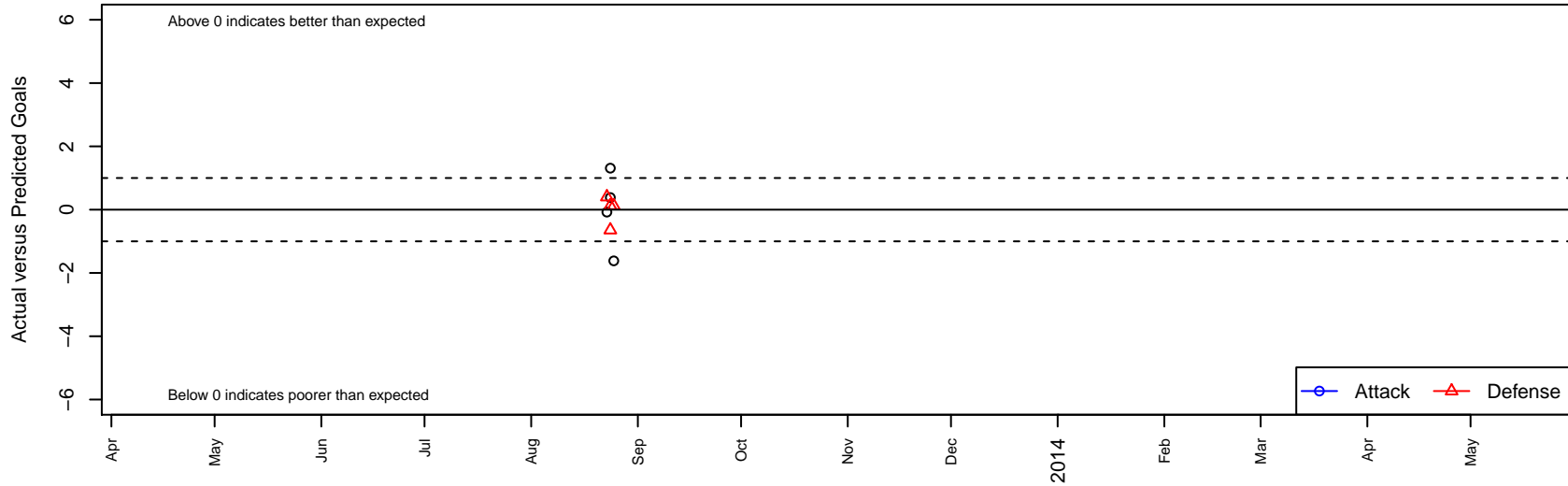
LCYSA Tsunami B98 Dots are actual minus expected GF (blue circles) and GA (red triangles). Blue line is smoothed change in attack strength. Red is smoothed change in defense strength.
